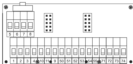
Connection 4-wire
